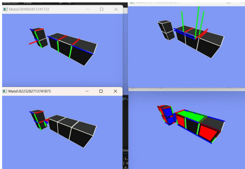
First attempt at feeding faces and the vanishing points to solvePnP. Bottom right image: classification of the edges and faces, top left, top right, bottom left images: solvePnP reference frame visualization of X faces, Y faces and Z faces, respectively.
