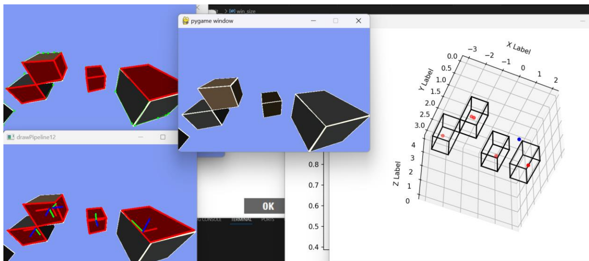
Another example of a successful analysis. All four cubes are reconstructed on the right.
