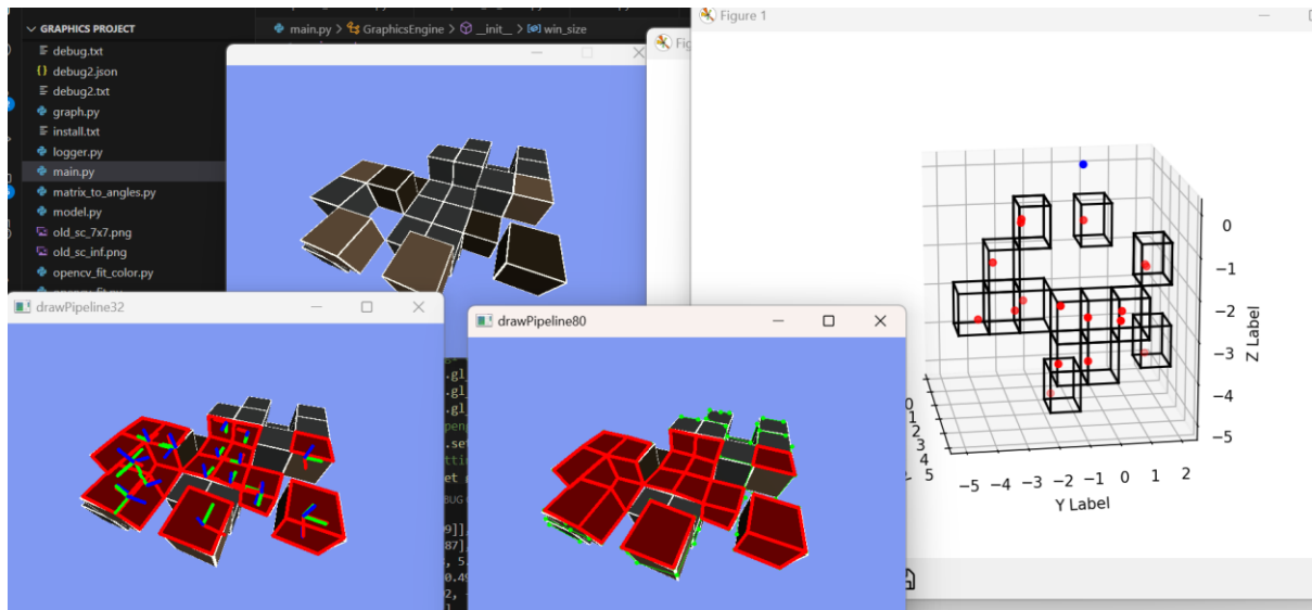
Example of a reconstruction of an image of cubes (top left) and and the result (diagram on the right). The blue dot represents the camera, this diagram is showing the result from under the camera. The other two auxiliary diagrams show which faces were recognized.
