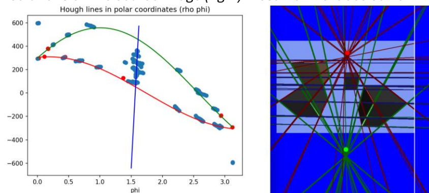
The vanishing points of the image above, in hough space(left) and on the source image (right)
