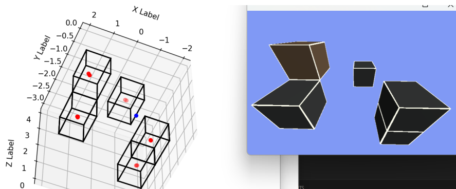
Running both solutions on the source image (right). Result of the faces solvePNP method (left)
